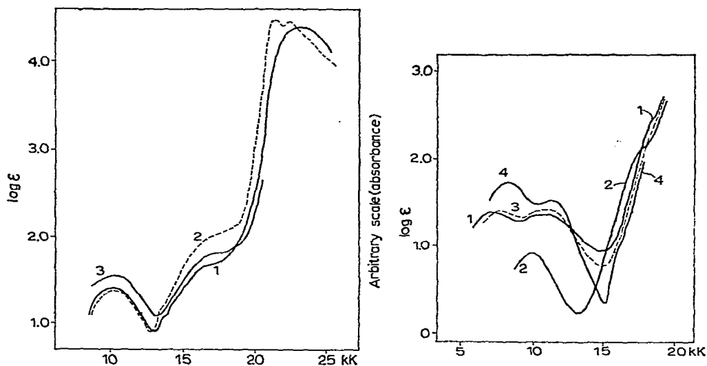
Fig. 2. Electronic spectra. (1) \text{Ni}(\text{sal.2-CH}_3\text{O.Ph})_2 in chloroform; (2) \text{Ni}(5,6\text{-benzo-sal.2-CH}_3\text{O.Ph})_2 in benzene; (3) \text{Ni}(5,6\text{-benzo-sal.2-CH}_3\text{O.Ph})_2 in the solid state (by reflectance).
